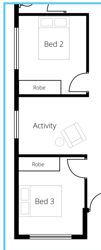
ALTERNATIVE BEDROOM / ACTIVITY ROOM LAYOUT
